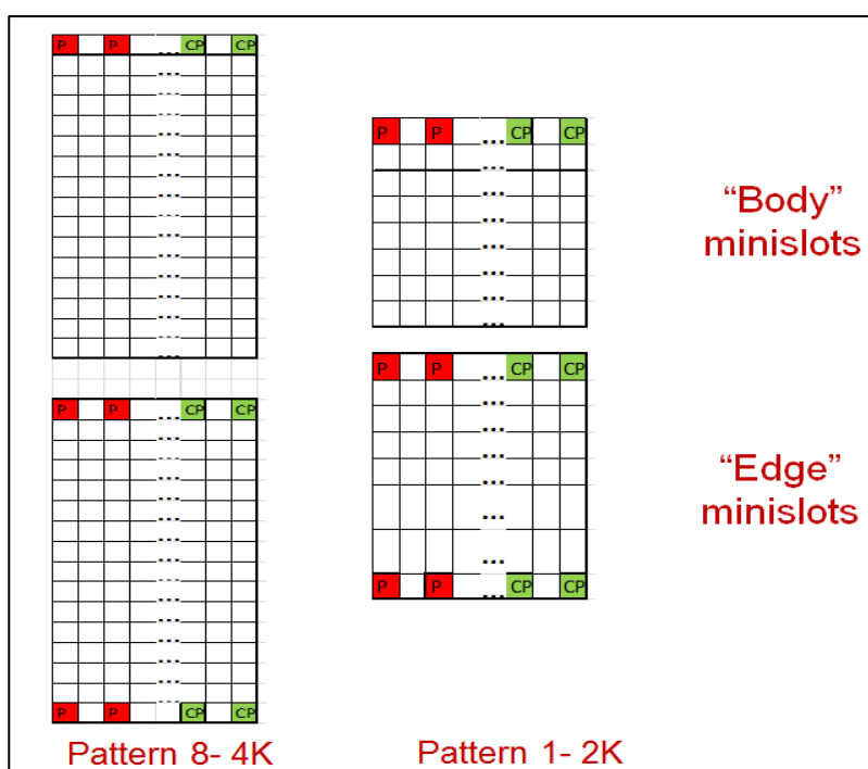
Figure 9. Pilot structures used for US spectral efficiency analysis
